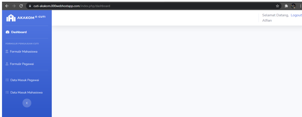
Gambar 2 Halaman Dashboard
