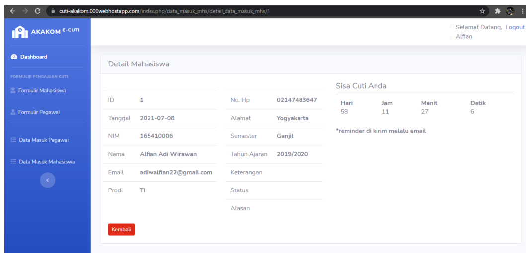
Gambar 5 Detail Data
