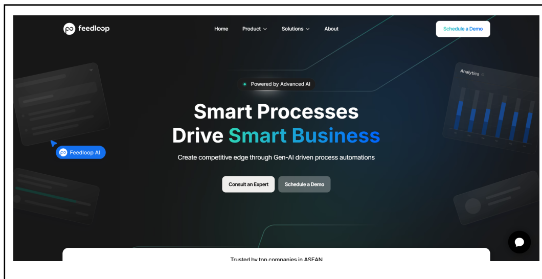
Gambar 2.1 Webpage Feedloop.ai
